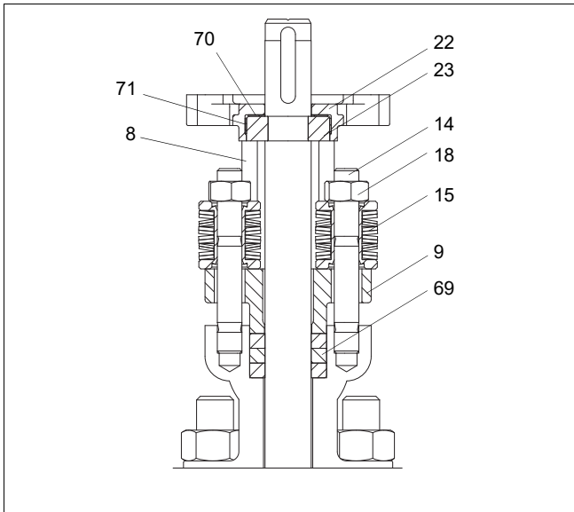
Fig. 6 Gland packing
