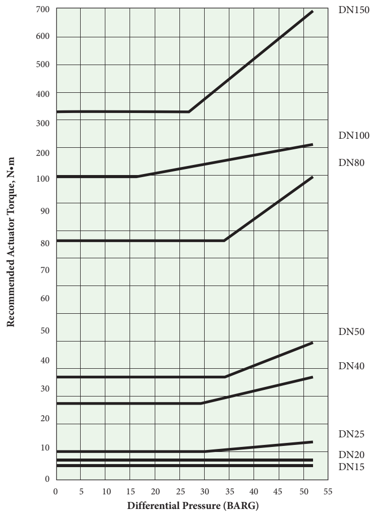
Valve Torque Data Xtreme (X) Seated Valves DIN 7000 Series, Reduced Bore, DN15 – DN50 Torque - Xtreme Seats
