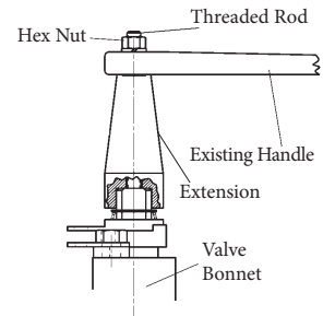
DN 80-150 Series 7000
